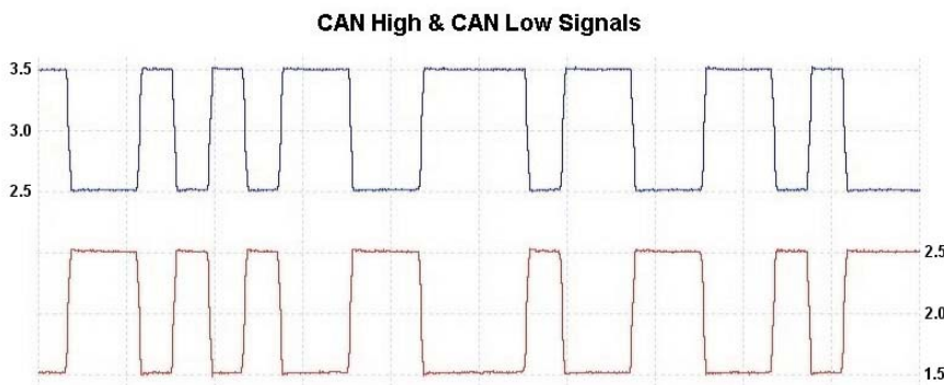
Fig 1 - CAN Electrical Signals
