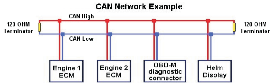
Fig 2 - CAN Network With Terminators
